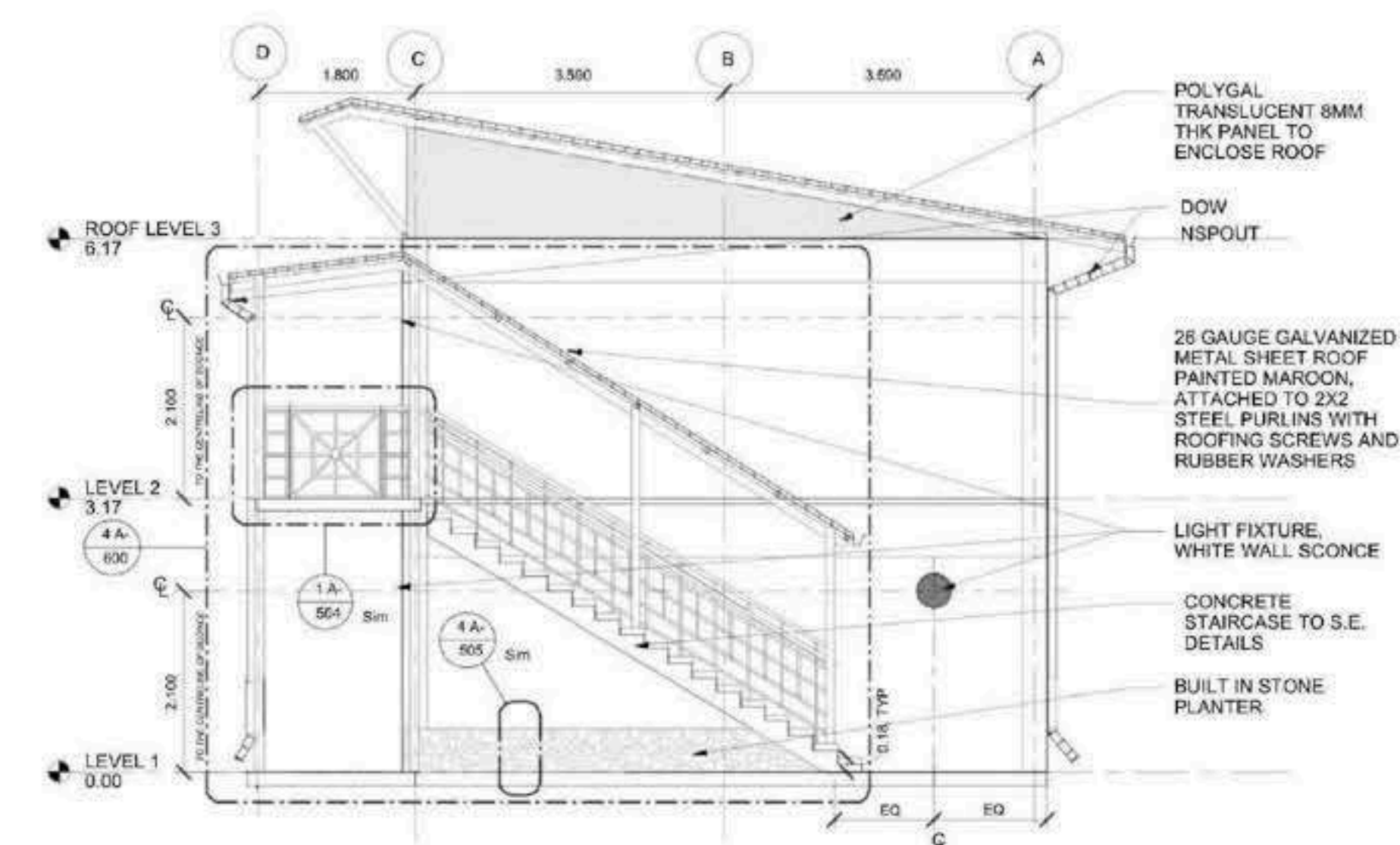
2 SIDE ELEVATION -2 CLASSROOM REGULAR
