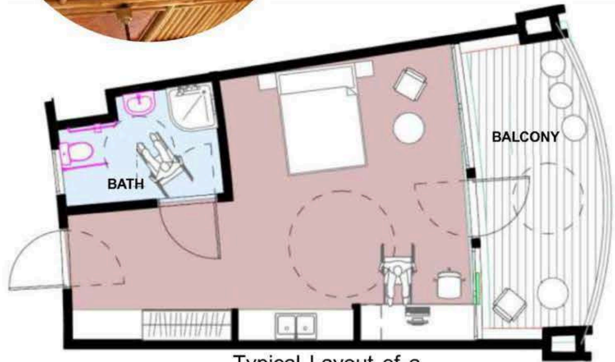
Typical Layout of a Paraplegic Room
